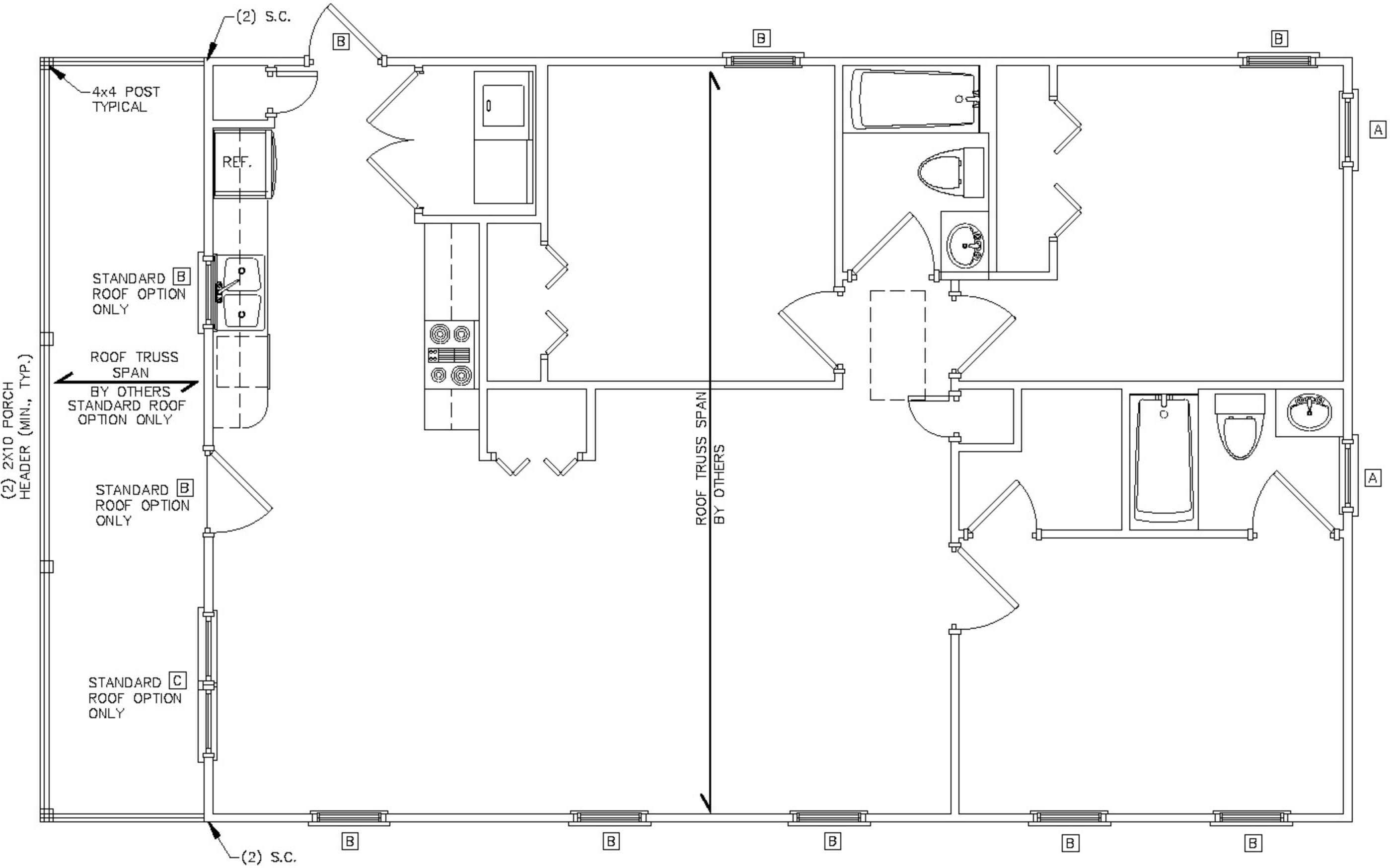
FRAMING PLAN
